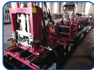
CNZ Roll Forming Machine
